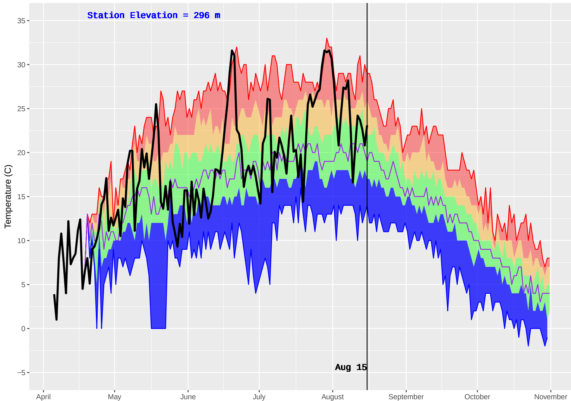
VAN DYKE (430) : Historical (1983–2016) and Current (2018) Daily Temperature
