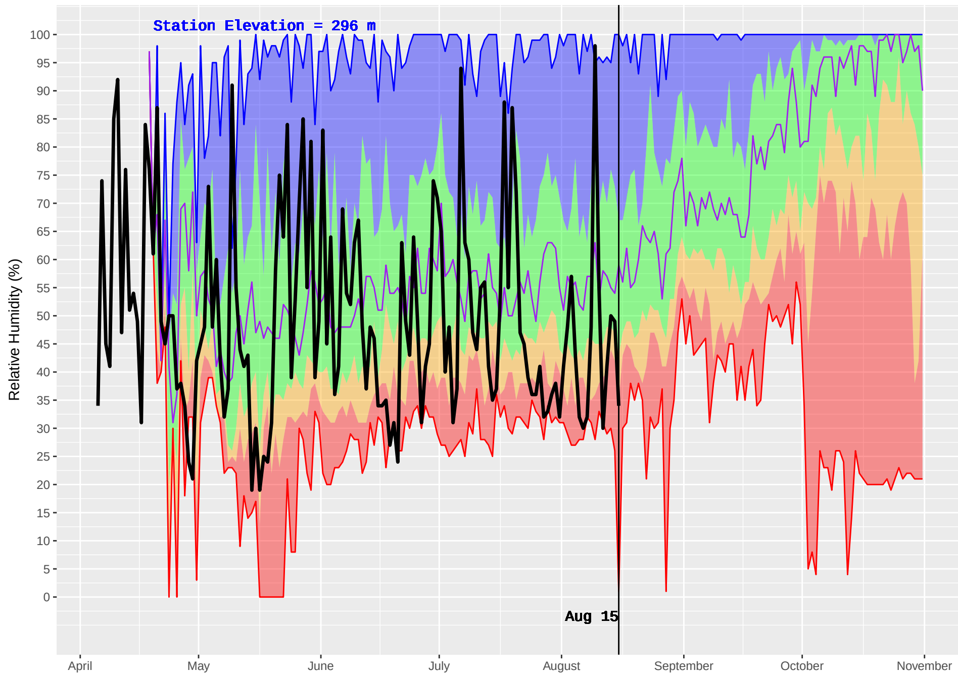
VAN DYKE (430) : Historical (1983–2016) and Current (2018) Daily Relative Humidity
